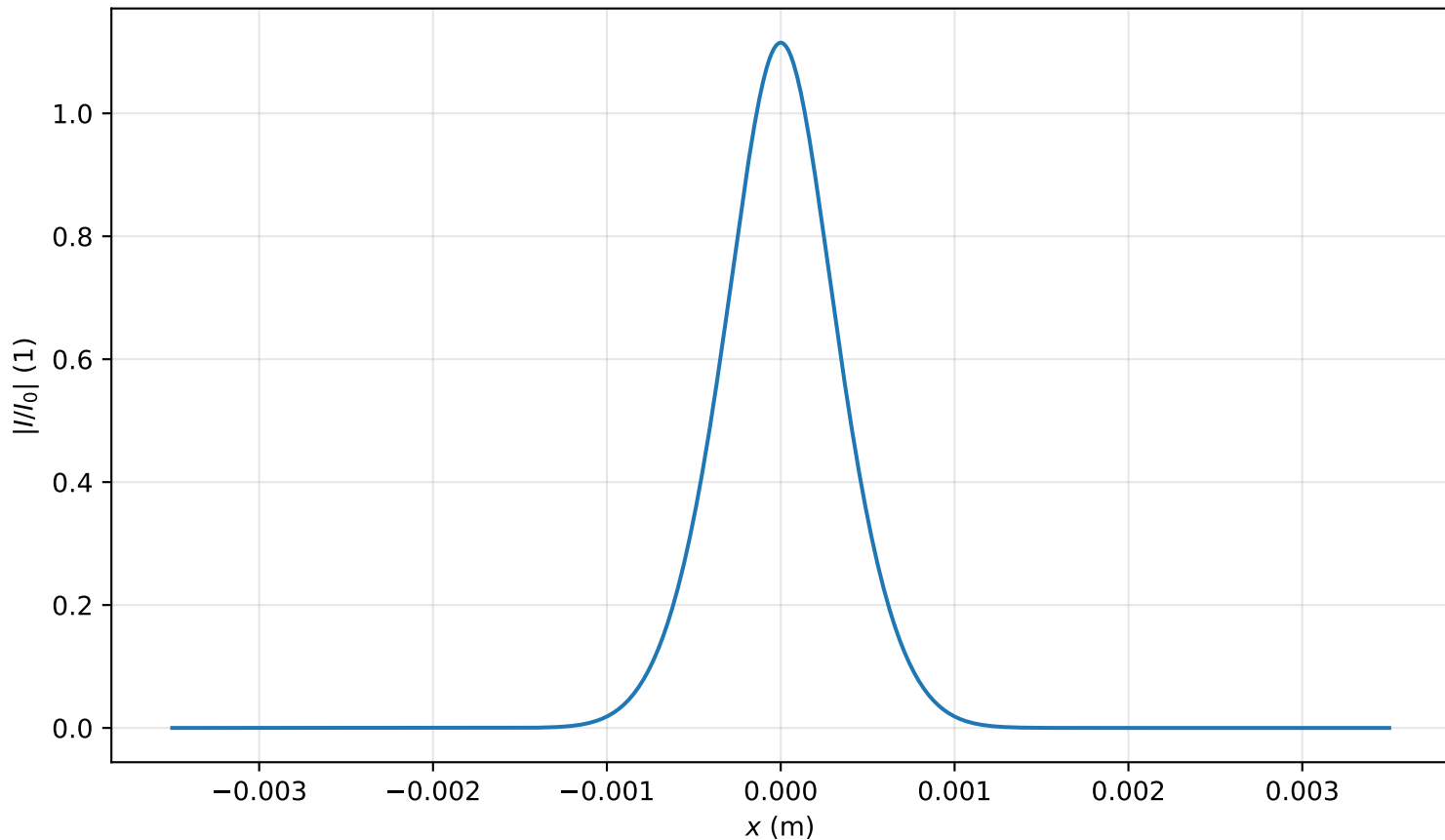
Intensity profile I(x, y = 0, z = 0.398m)/I_0 , P_{in}=1.0P_{cr} , artificial time
